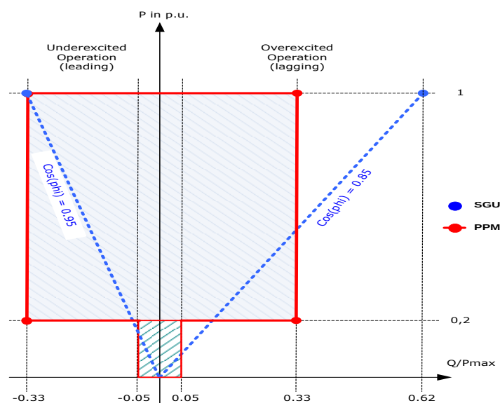
Figure 2.1 P-Q Diagram
