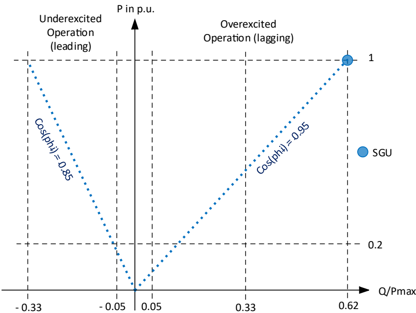
Figure 6: P-Q Diagram (Synchronous)
