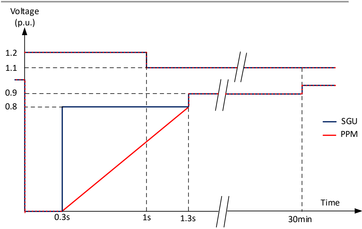
Figure 5: Voltage Operate through Capability Diagram (PPM)
