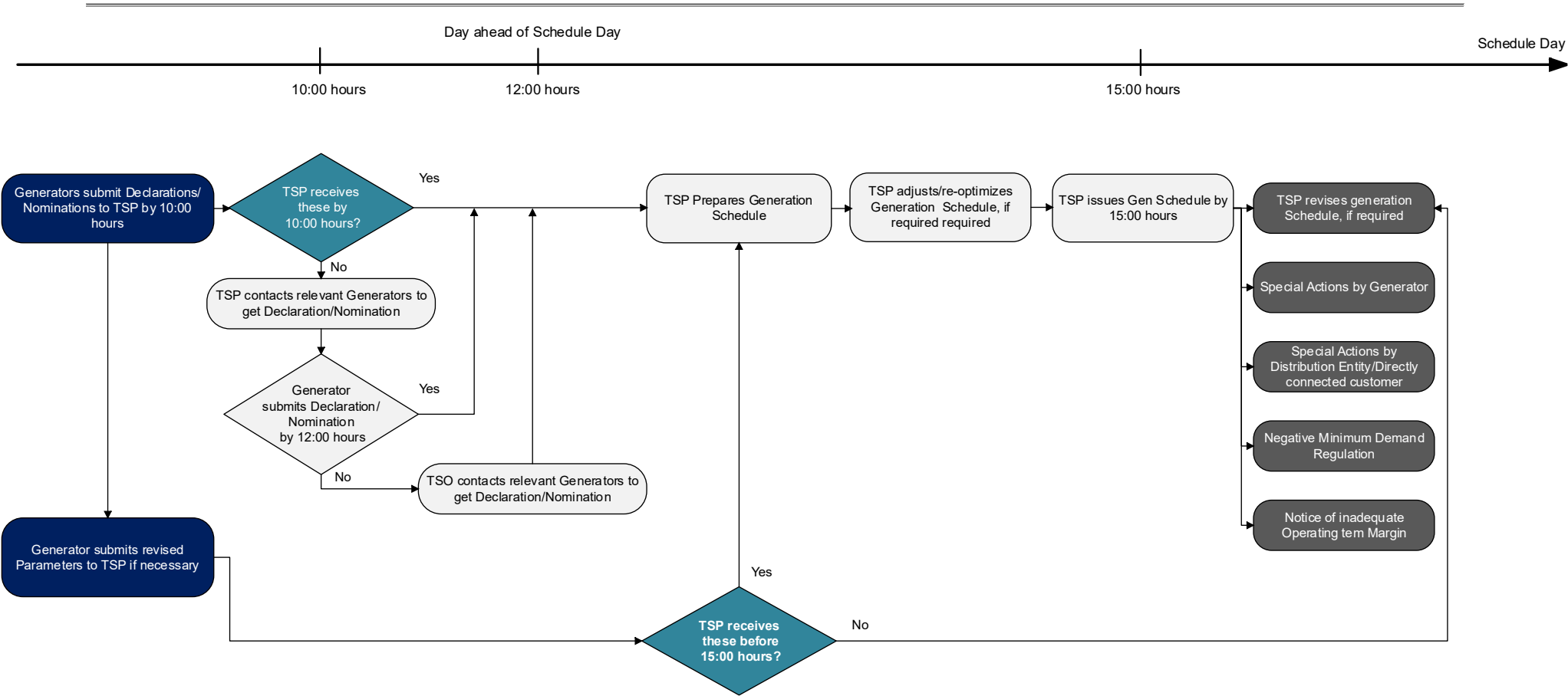
Figure 14: Overview of generation scheduling process
