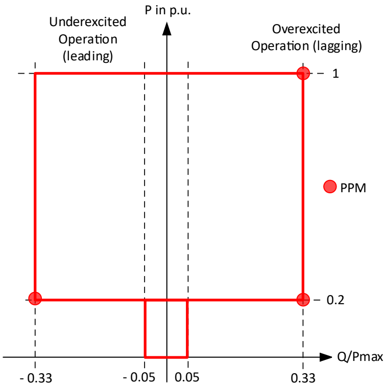
Figure 4: P-Q Diagram (PPM)
