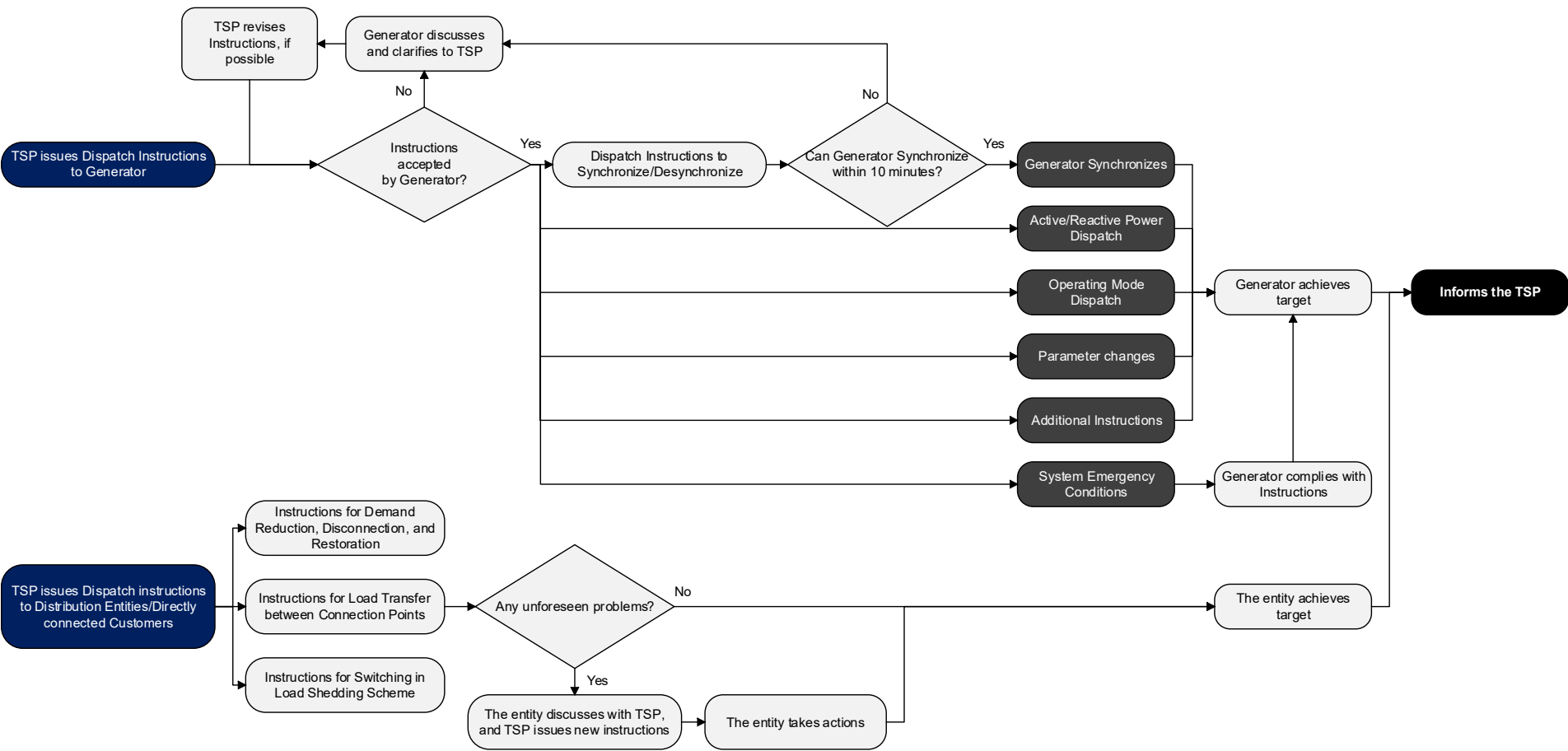
Figure 15: Overview of the dispatch process
