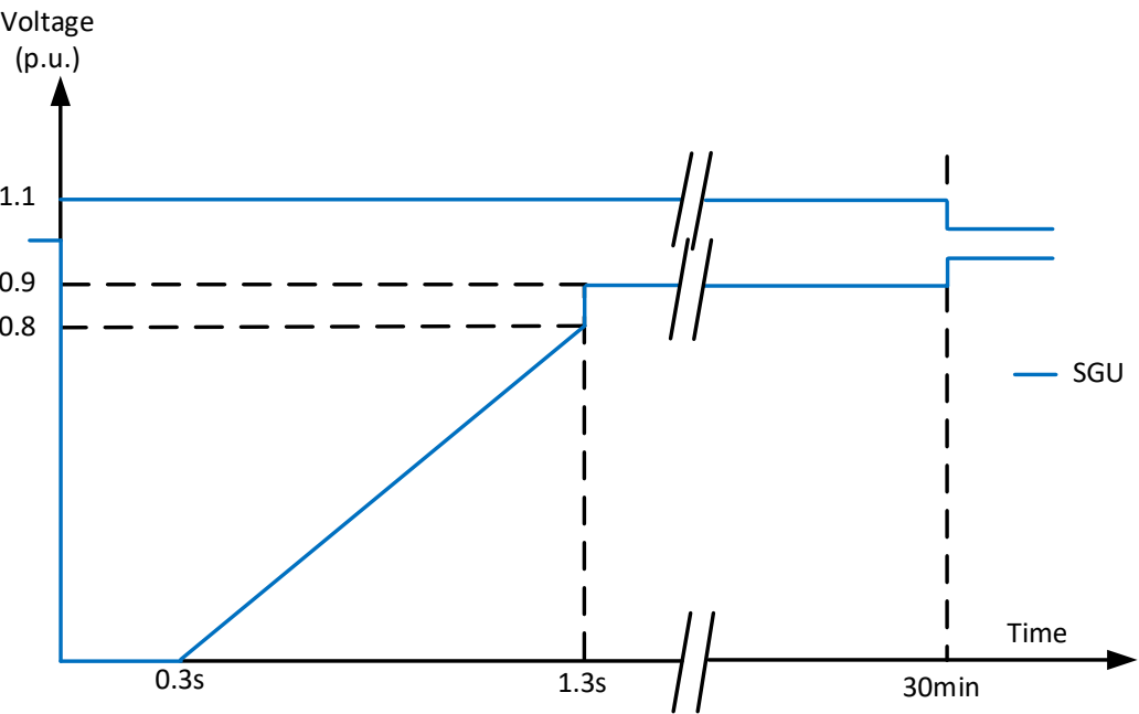
Figure 7: Voltage Operate through Capability Diagram (Synchronous)
