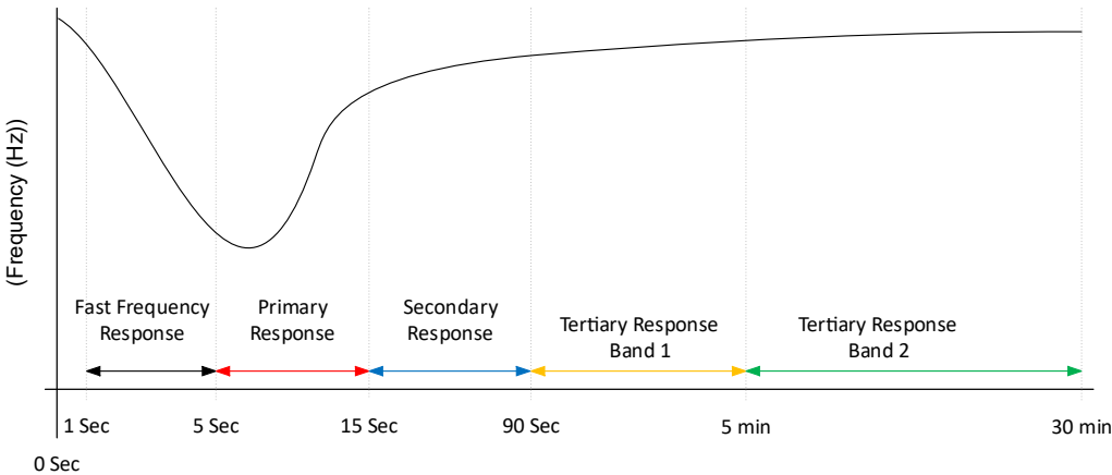
Figure 10: Operating Reserve and Frequency Control Timeframes
