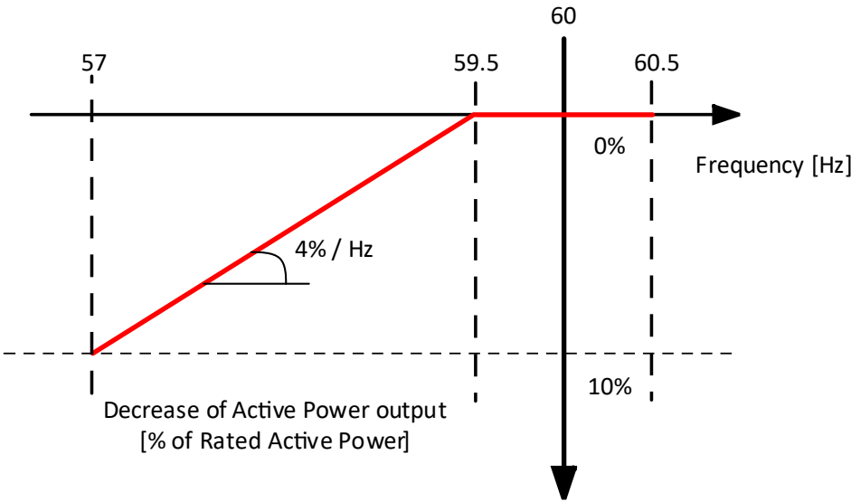
Figure 3: Maximum Output Power Reduction Diagram
