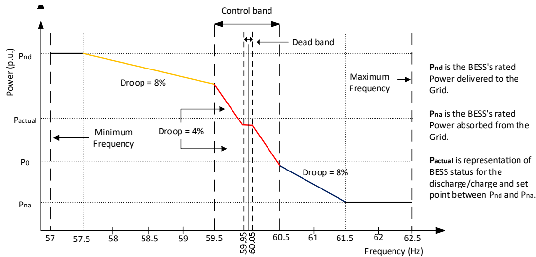
Figure 9: BESS response during normal, high, and low frequency
