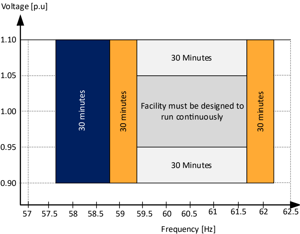
Figure 8: Normal operating range: Asynchronous facilities, 110-380 kV
