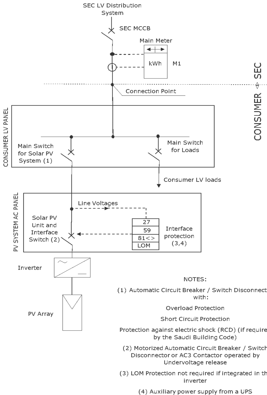
Figure 11- LV Connection Scheme – Case of Two (or more) Main Switches in absence of one general Main Switch in the incomer from SEC. (case as per Figure 9 shown, but this applies to both schemes of Figure 9 and Figure 10)
