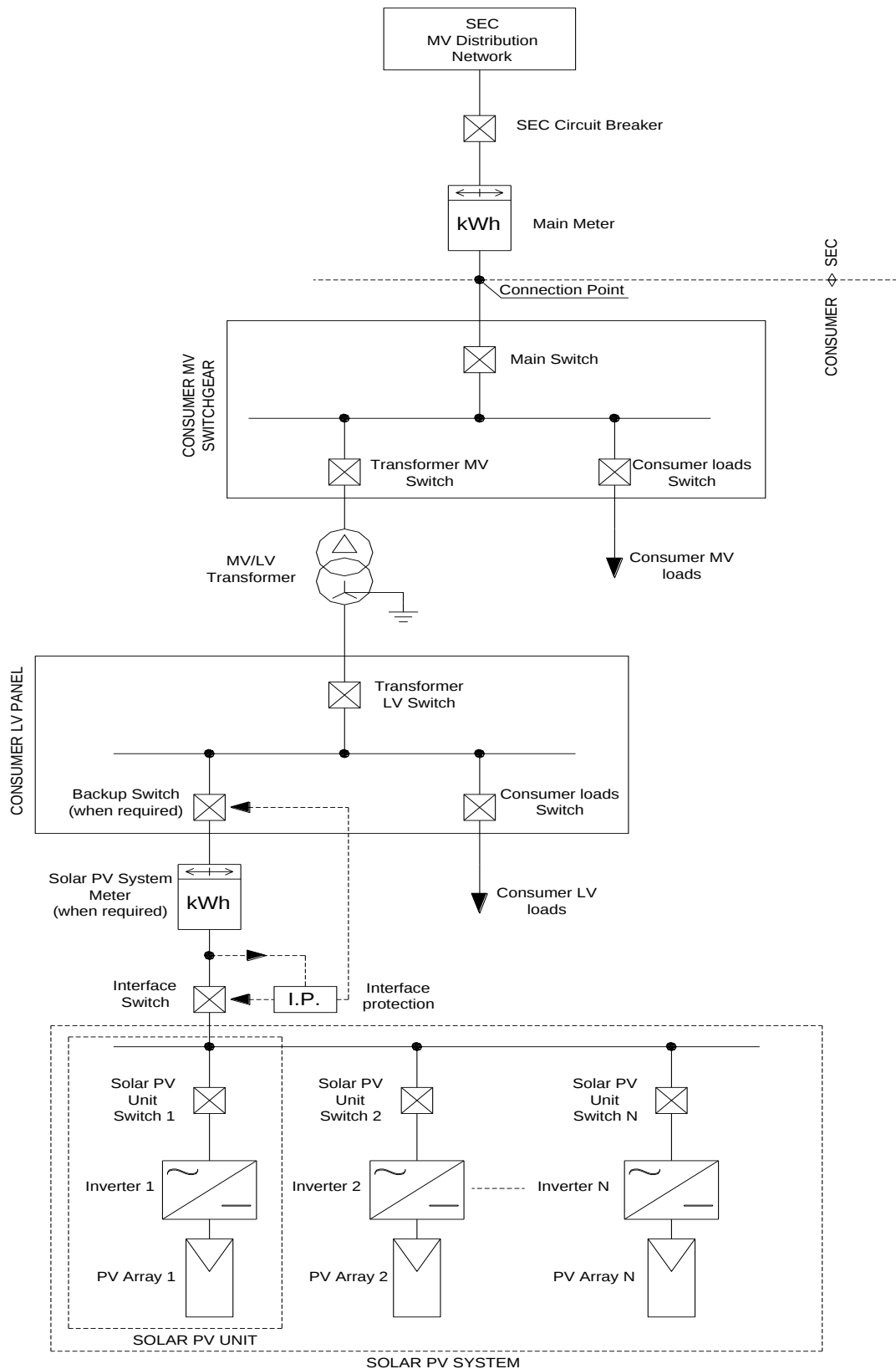
Figure 2 - Schematic representation for the interconnection of a Small-scale Solar PV System with SEC MV Distribution Network (either 13.8 or 33kV)
