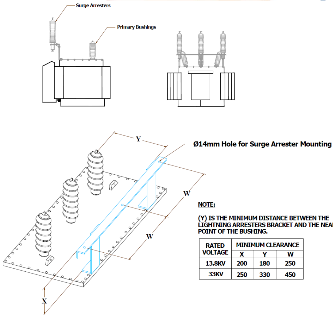
Figure 1: Surge arresters mounting bracket for pole-mounted transformers
