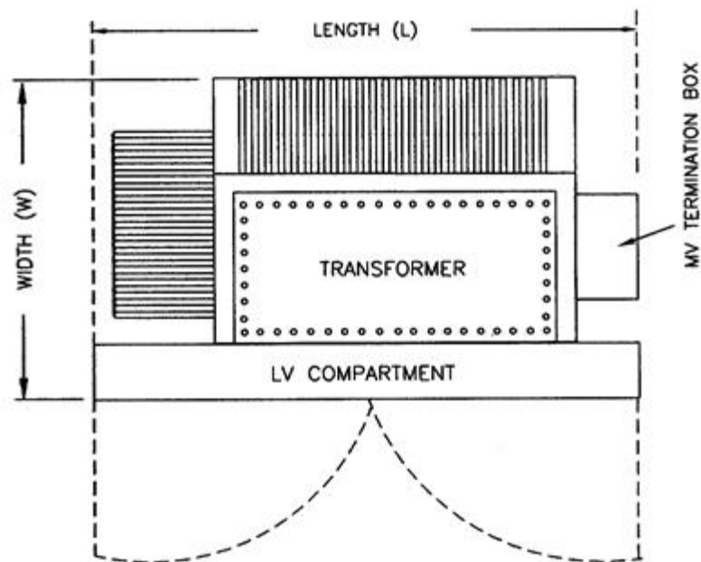
Figure 1: Unit Substation component lay-out.
